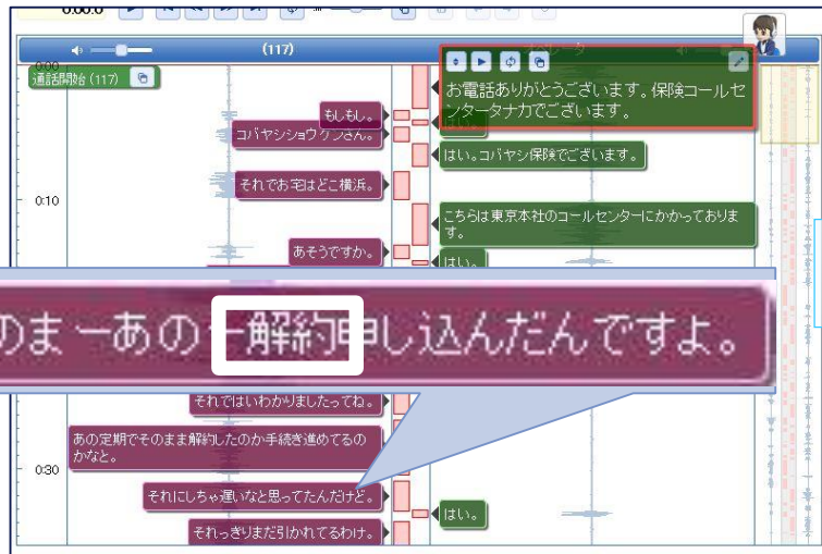
Amivoice SpeechVisualizer
